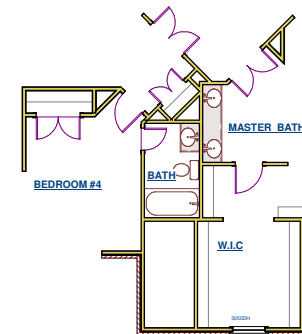
2ND FLOOR PLAN ELEVATION A / E OPTIONAL BEDROOM #4 BATH AND OPTIONAL HALF BATH
