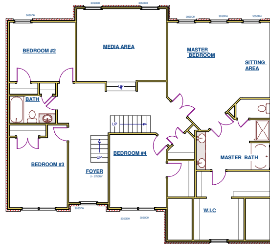
2ND FLOOR PLAN - ELEVATION C
