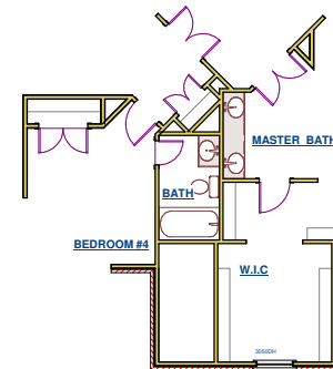
2ND FLOOR PLAN ELEVATION B OPTIONAL 4 BEDROOM BATH W/ OPTIONAL HALF BATH
