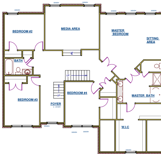
2ND FLOOR PLAN - ELEVATION C W/ OPTIONAL HALF BATH
