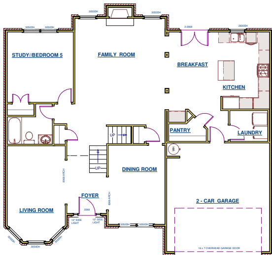
FIRST FLOOR PLAN - ELEVATION A / E
