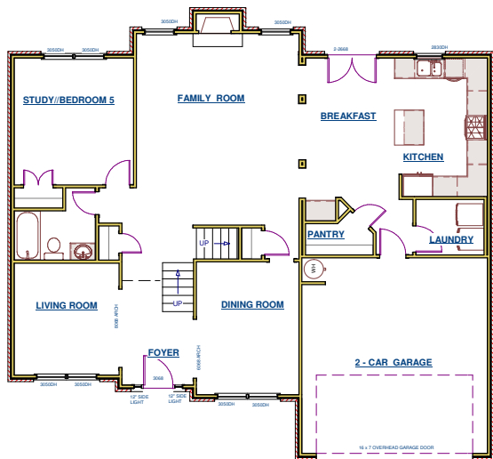
FIRST FLOOR PLAN - ELEVATION B
