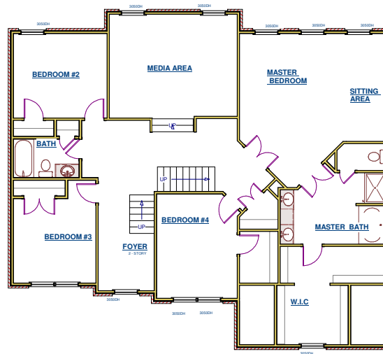
2ND FLOOR PLAN - ELEVATION B
