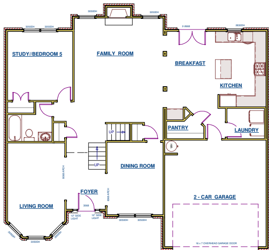
FIRST FLOOR PLAN - ELEVATION D/F
