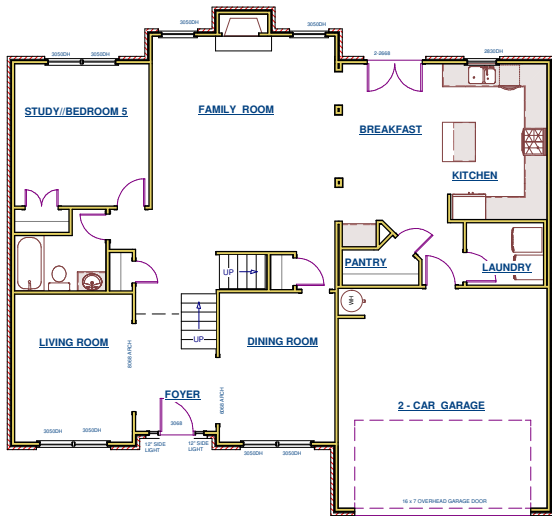
FIRST FLOOR PLAN - ELEVATION C
