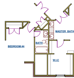
2ND FLOOR PLAN ELEVATION A / E OPTIONAL BATH
