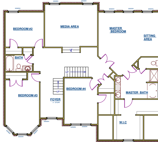
2ND FLOOR PLAN - ELEVATION A / E
